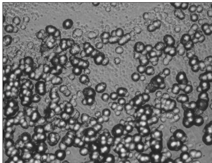
One of Dr. Kowalski's photomicrographs. He noted the two different sizes of pits in the CR-39 detectors. He concluded that the larger pits could not be from cold fusion radiation (LCF #319).
