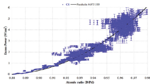
FIGURE 5. Effect of D/Pd ratio on the measured power at 20° C reported by McKubre et al.[28] when the electrolytic method is used. The behavior is obtained using a single batch of Pd metal that contained some NAE.
