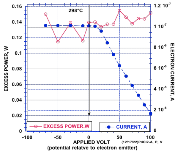
FIGURE 15. Effect of a voltage applied between the emitter and collector on the electron current at 298^\circ\text{C} , based on the behavior plotted in Fig 14. The excess power is also shown. The voltage polarity is such that electrons with less than the plotted voltage are caused to return to the electrode surface, hence are not measured as an emitted current.
